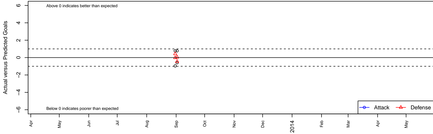
GHYSA Real Pacific B95 Dots are actual minus expected GF (blue circles) and GA (red triangles). Blue line is smoothed change in attack strength. Red is smoothed change in defense strength.
